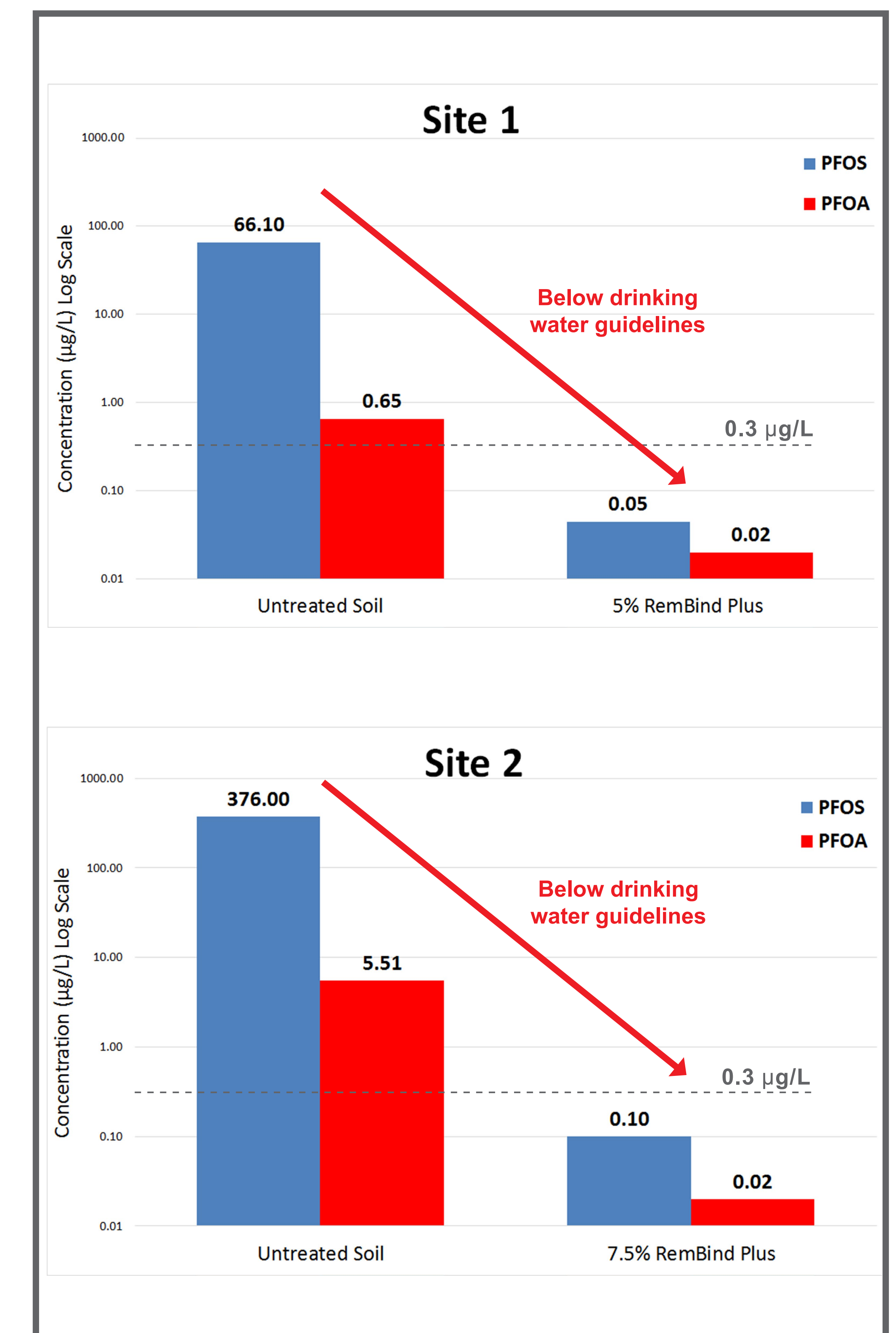
Figure 1: PFOS and PFOA leachability at pH 5 for various RemBind Plus treatments. The grey line indicates the Minnesota Department of Health Drinking Water Guideline value of 0.3 µg/L.
